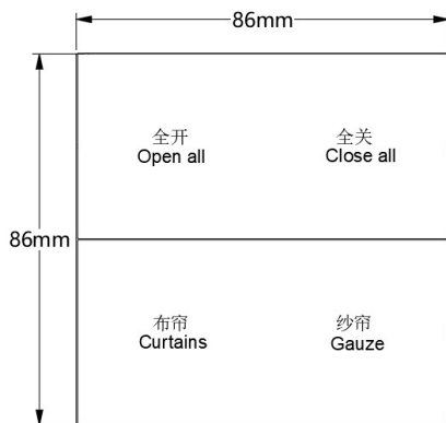
MK1204 dimensional drawing
